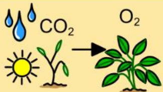
photosynthesis
