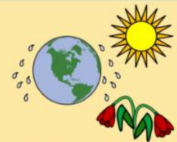
global warming
