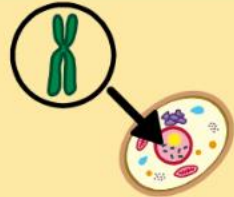
chromosomes
