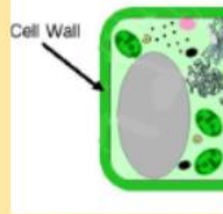
cell walls
