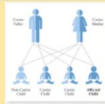
genetics
